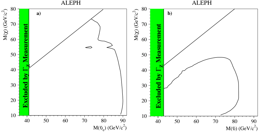
Fig. 13. a The 95% C.L. limit in the (M_\chi, M_{\tilde{\nu}_e}) plane for \tilde{\nu}_e decaying indirectly via a dominant \bar{U}\bar{D}\bar{D} operator. The \tilde{\nu}_e cross-section is evaluated in the region \mu = -200 GeV/c 2 and \tan\beta = 2 . (The non-excluded island near M_{\tilde{\nu}_e} = 70 GeV/c 2 is excluded at 90% C.L.) b The exclusion obtained assuming three mass degenerate sneutrinos
