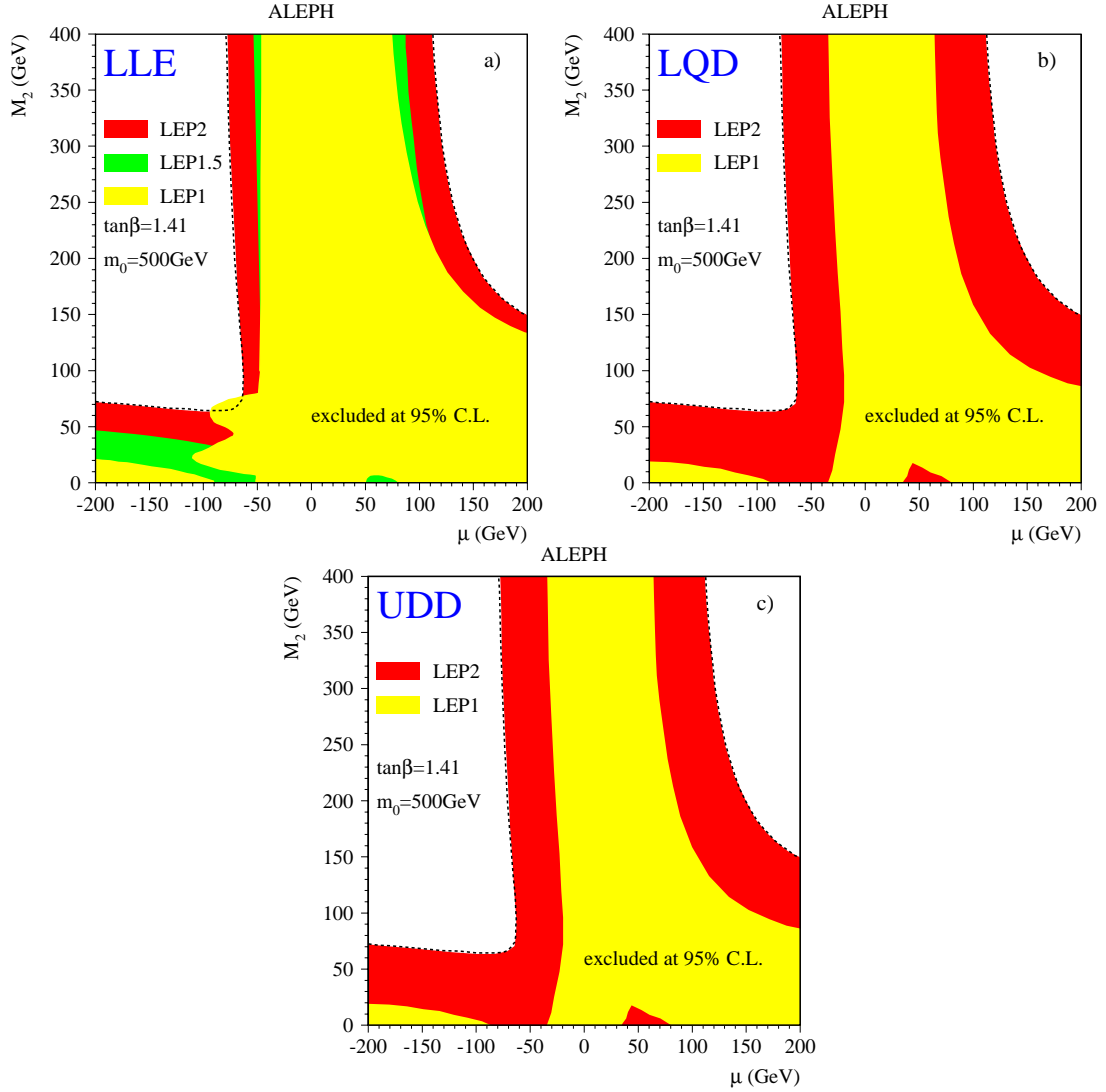
Fig. 2. Regions in the (\mu, M_2) plane excluded at 95% C.L. at \tan\beta = 1.41 and m_0 = 500 \text{ GeV}/c^2 for the three operators. The dotted line is the kinematic limit for the pair production of the lightest chargino. The black region is the exclusion obtained using the 183 GeV data. The light grey region is the exclusion from the LEP 1 data. The dark grey region in Fig. 2a is excluded using the 130-136 GeV (LEP 1.5) data[5]
