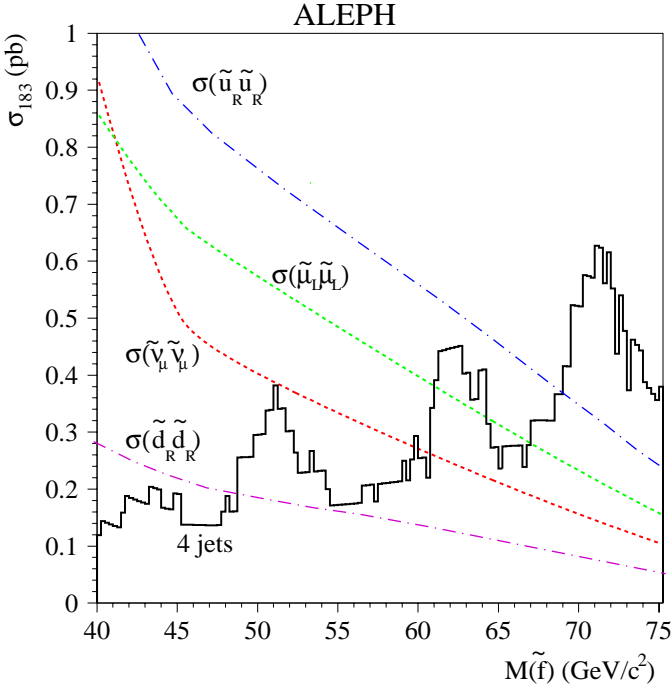
Fig. 8. The 95% C.L. excluded cross-sections scaled to \sqrt{s} = 183 GeV for sleptons (via LQ\bar{D} ), sneutrinos (via LQ\bar{D} ) and squarks (via \bar{U}D\bar{D} ) decaying directly to four jets. The MSSM cross-sections for pair production of muon sneutrinos, left-handed smuons and right-handed squarks are superimposed
