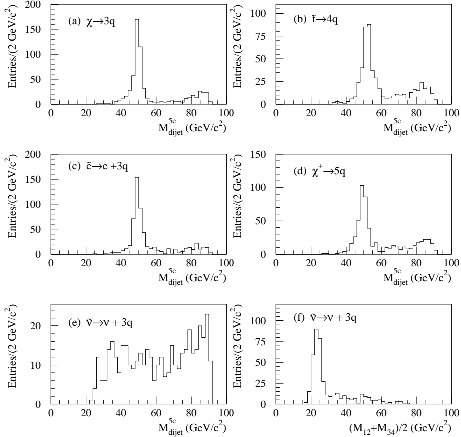
Fig. 9. Mass reconstruction for various \bar{U}\bar{D}\bar{D} decay topologies: Dijet mass distribution of events (forced to 4 jets), after the 5C fit, for boosted pairs of sparticles ( M_{\tilde{f}} = 50 \text{ GeV}/c^2 , M_{\chi} = 25 \text{ GeV}/c^2 ). a 6 quarks, b 8 quarks, c 6 quarks + 2 leptons, d 10 quarks, e 6 quarks + 2 \nu . As can be seen from e , in the presence of missing energy the mass reconstruction for the sneutrino, using the 5C fit, no longer works. For this case, using the sum of dijet masses before the 5C fit f allows reconstruction of the \chi mass instead
