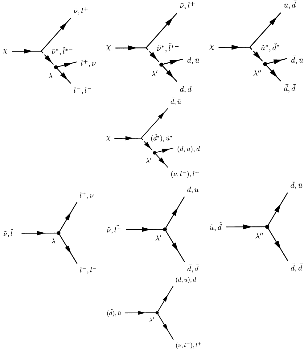
Fig. 1. Direct R-parity violating decays of supersymmetric particles via the \lambda , \lambda' and \lambda'' couplings. The black dot marks the R-parity violating vertex in the decay
