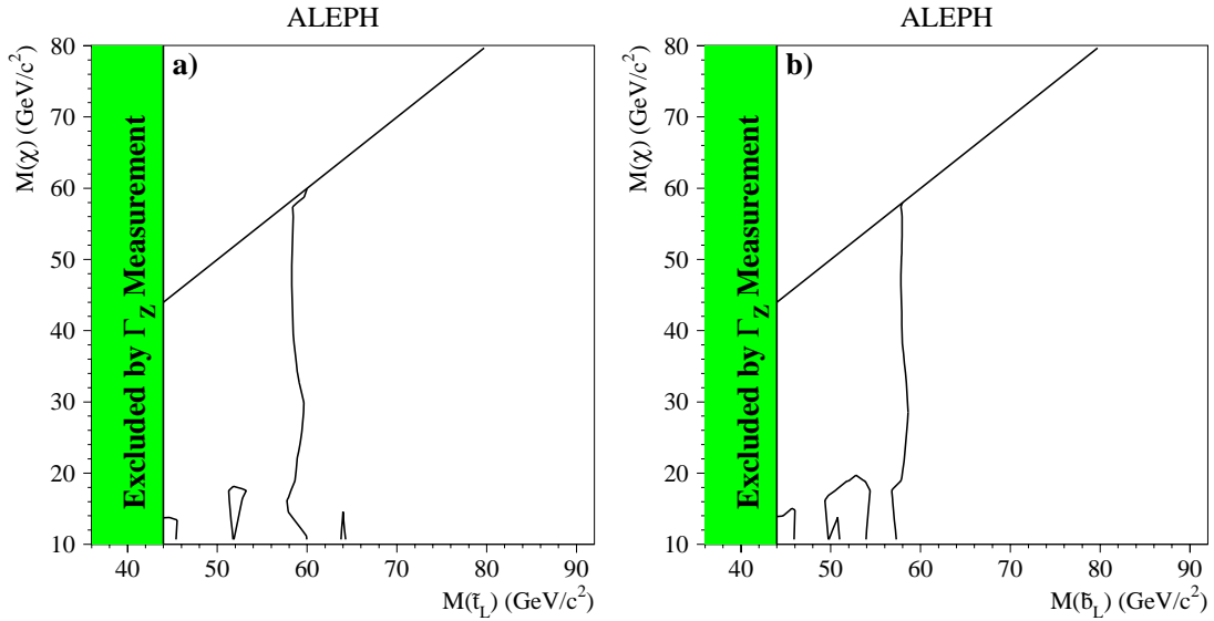
Fig. 11. The 95% C.L. exclusion for squarks decaying indirectly via a dominant \bar{U}\bar{D}\bar{D} operator: a left-handed stop, b left-hand sbottom. (The non-excluded regions for neutralino masses less than 20 \text{ GeV}/c^2 are excluded at 90% C.L.)
