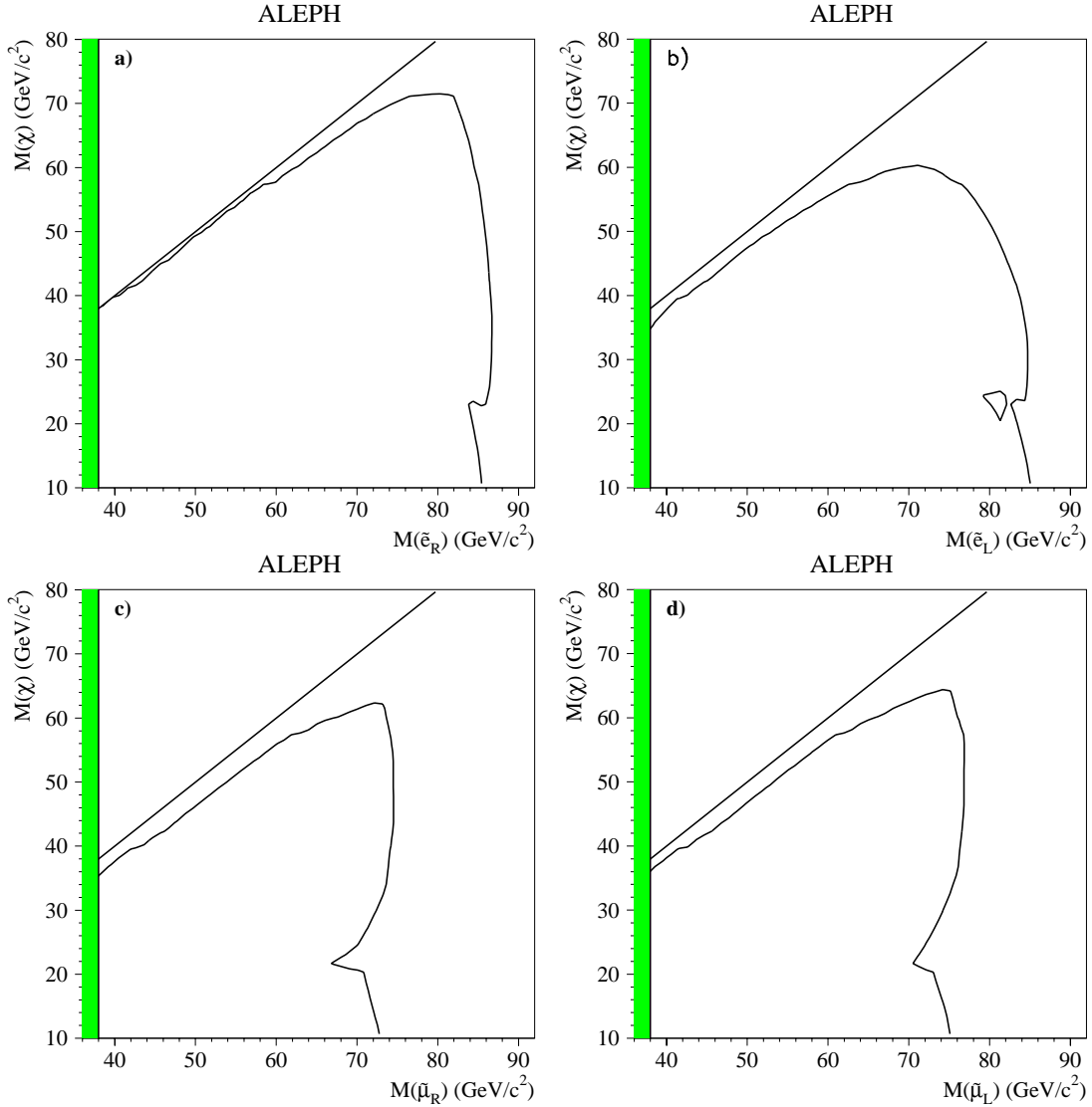
Fig. 12. The 95% C.L. excluded cross-sections for left or right-handed selectrons and smuons decaying indirectly via a dominant \bar{U}\bar{D}\bar{D} operator. The selectron cross-section is evaluated in the region \mu = -200 \text{ GeV}/c^2 and \tan\beta = 2
