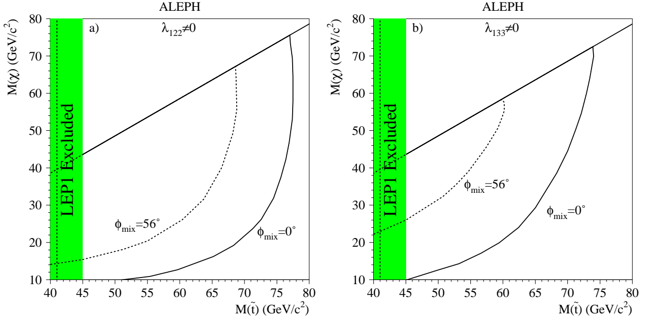
Fig. 3. The 95% C.L. limits in the (M_\chi, M_{\tilde{t}}) plane for indirect stop decays via a LL\bar{E} couplings a) \lambda_{122} and b) \lambda_{133} . The two mixing angles chosen correspond to the best and worst case cross-sections. The LEP 1 limit for \phi_{\text{mix}} = 0^\circ (and \phi_{\text{mix}} = 56^\circ -dashed line) is also shown
