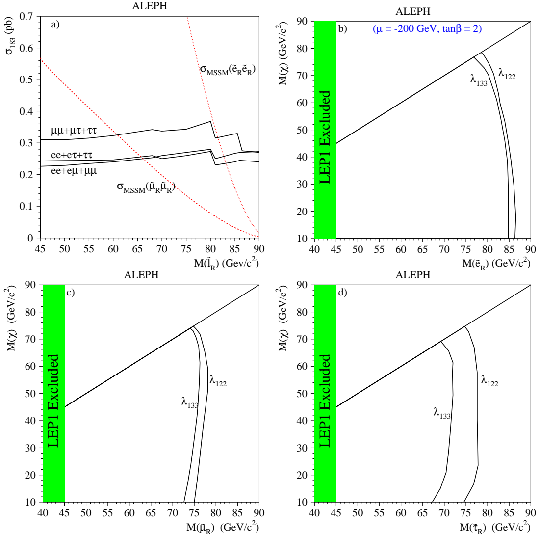
Fig. 4. a The 95% C.L. exclusion cross-sections scaled to \sqrt{s} = 183 GeV for sleptons decaying directly via a dominant LL\bar{E} operator. For the purpose of this plot a \beta^3/s cross-section dependence was assumed. The dashed line shows the MSSM cross-section for pair production of right-handed smuons, the dashed-dotted the cross-section for right-handed selectrons at \tan\beta = 2 , \mu = -200 GeV/c 2 , M_2 = 50 GeV/c 2 . Figs b , c and d show the 95% C.L. limits in the (M_\chi, M_{\tilde{l}}) plane for selectrons, smuons and staus decaying indirectly via a dominant LL\bar{E} operator. The two choices of \lambda_{122} and \lambda_{133} correspond to the best and worst case exclusions respectively. The selectron cross-section is evaluated in the gaugino region at \mu = -200 GeV/c 2 , \tan\beta = 2
