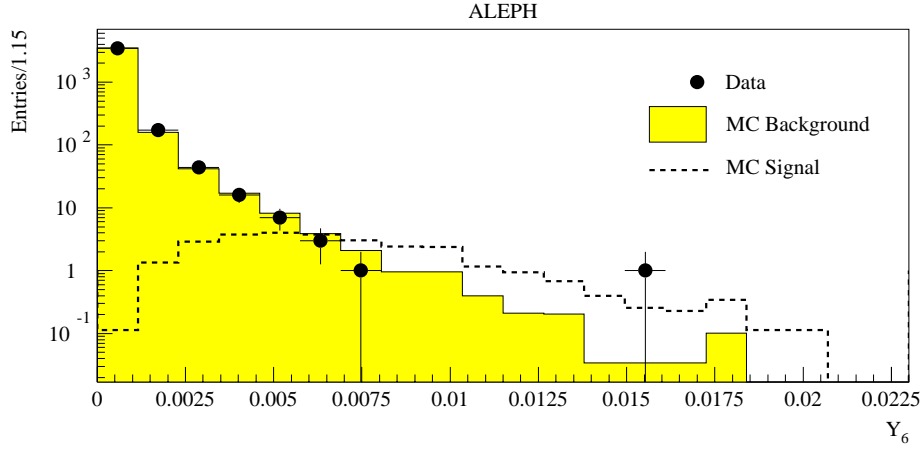
Fig. 10. Data/Monte Carlo comparison of the Durham y_6 distance. The dashed line is the expected signal for \chi^+\chi^- ( M_{\chi^+} = 90 \text{ GeV}/c^2 ) decaying indirectly via a \bar{U}\bar{D}\bar{D} operator to \chi ( M_\chi = 40 \text{ GeV}/c^2 ), assuming a production cross-section of 0.5 \text{ pb}
