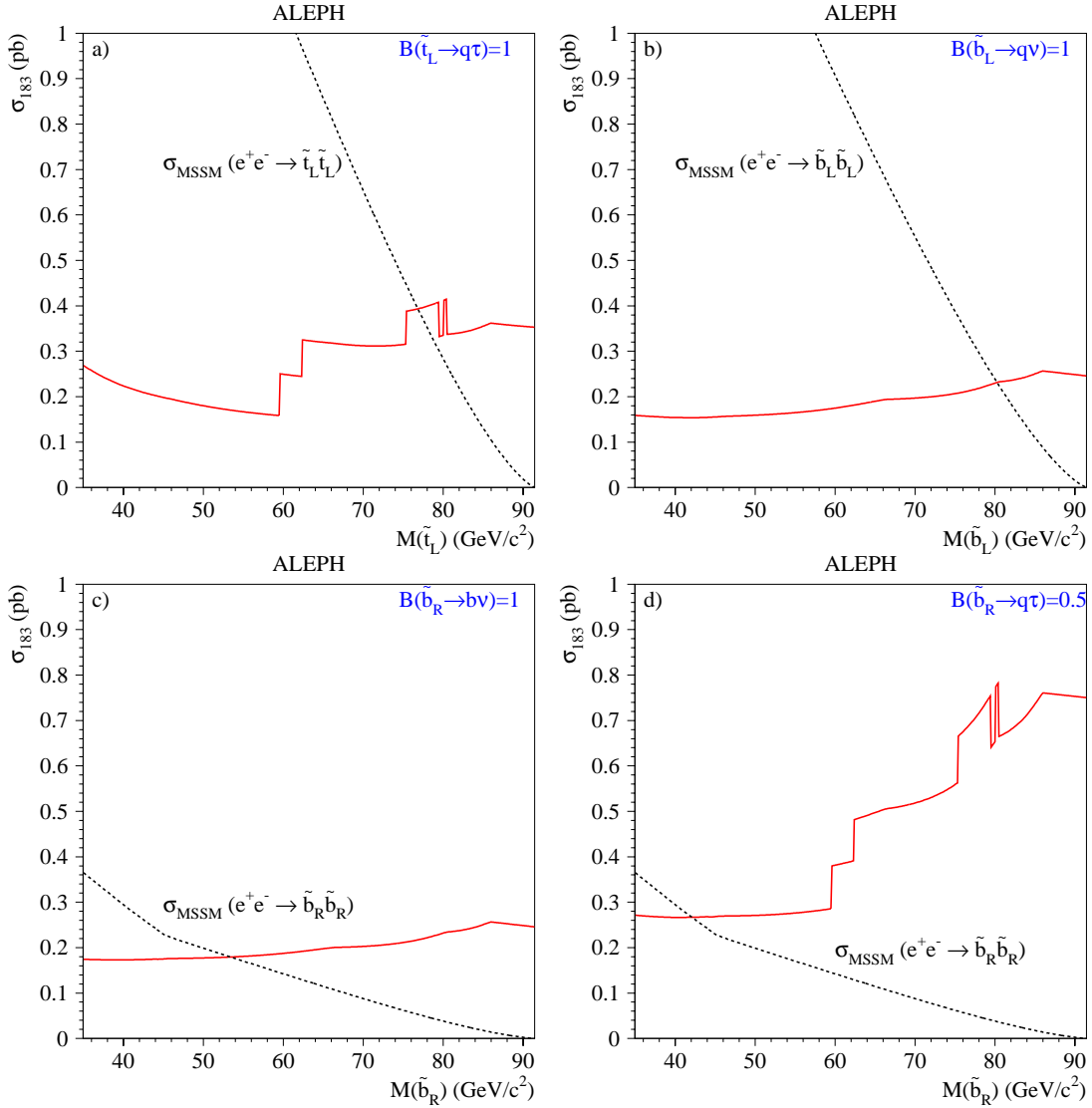
Fig. 6a–d. The 95% C.L. excluded cross sections for the direct squark decays via a dominant LQ\bar{D} operator: a \tilde{t}_L\tilde{t}_L \rightarrow \tau q\tau q , b \tilde{b}_L\tilde{b}_L \rightarrow q\nu q\nu , c \tilde{b}_R\tilde{b}_R \rightarrow b\nu b\nu and d \tilde{b}_R production with a 50% branching ratio into q\tau and q\nu . The MSSM cross sections are superposed as dashed lines
