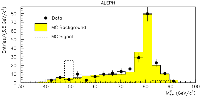
Fig. 7. Data/Monte Carlo comparison of the reconstructed dijet mass after forcing the event to four jets and performing the 5C fit. The dashed line is the signal for 50 GeV/c 2 left-handed selectrons decaying directly via the LQ\bar{D} coupling, normalised to a cross-section of 2.4 pb
