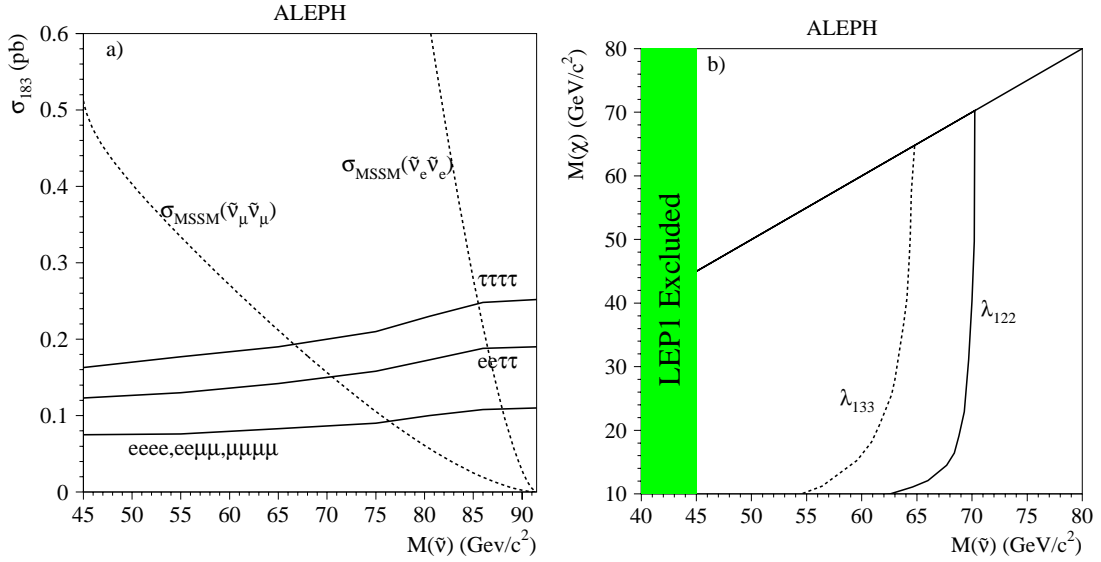
Fig. 5. a The 95% C.L. exclusion cross-sections scaled to \sqrt{s} = 183 GeV for sneutrinos decaying directly via a dominant LL\bar{E} operator. For the purpose of this plot a \beta^3/s cross-section dependence was assumed. The MSSM cross-sections ( \tan\beta = 2 ) for pair production of electron sneutrinos ( \mu = -200 GeV/c 2 , M_2 = 100 GeV/c 2 ) and muon sneutrinos are superimposed. b The 95% C.L. limits in the (M_\chi, M_{\tilde{\nu}}) plane valid for indirect \tilde{\nu}_\mu and \tilde{\nu}_\tau decays. The limits for \tilde{\nu}_e are always at least as stringent as those presented. The two choices of \lambda_{122} and \lambda_{133} correspond to the best and worst case exclusions respectively
